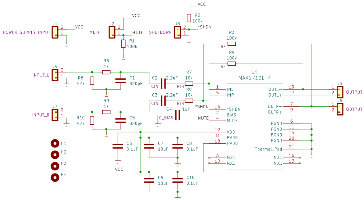
Figure 1. AMP2X1 schematic.
