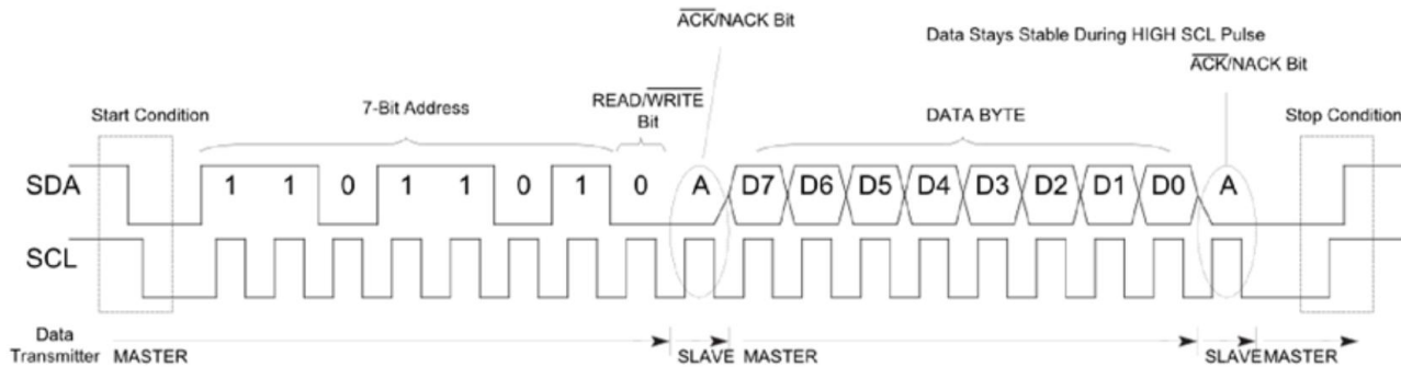
Figure 8. I²C Write Sequence Transmission
